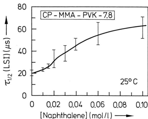
Fig. 1. \tau_{1/2} (LSI) versus the concentration of naphthalene added to an acetone solution of a poly(methylmethacrylate-co-phenylvinylketone) sample containing 7.8 mol% PVK (0.021 base mol/l). Absorbed dose per flash: 8.4 \times 10^{-5} einstein/l.
